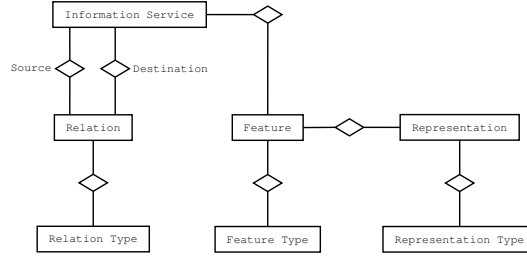
Figure 1: Typing of Relations, Features and Representations
